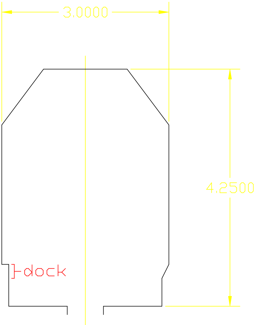
□n30 clearance gauge (based on NMRA □n3)
